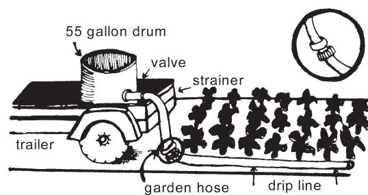
Figure 10. Trickle system for a garden that is too far from a water supply.
