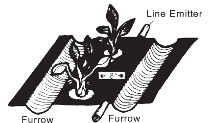
Figure 14. Installation of trickle irrigation under black plastic mulch.
